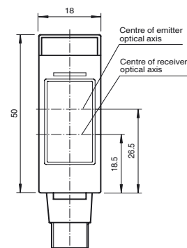
Unit connector
